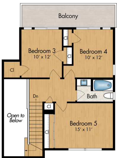
Upper Level
